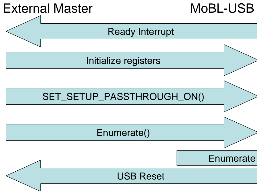
Figure 4-3. Passthrough Enumeration
