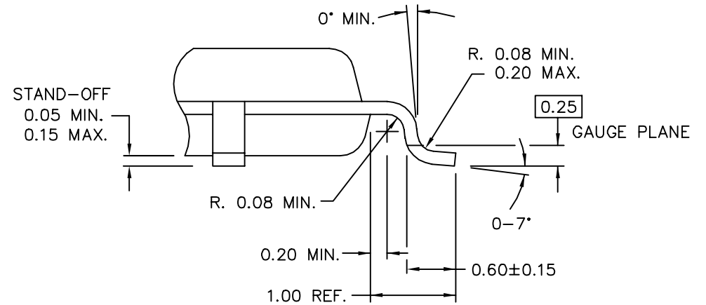
DETAIL A
