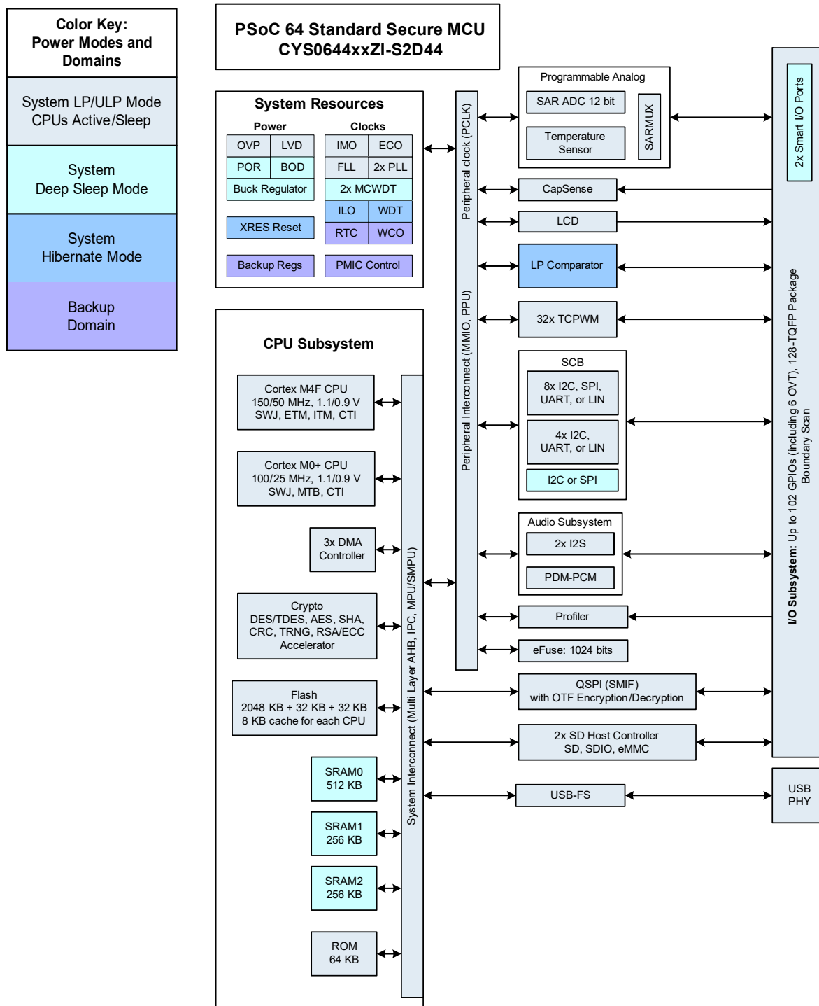
Figure 2. Block Diagram
