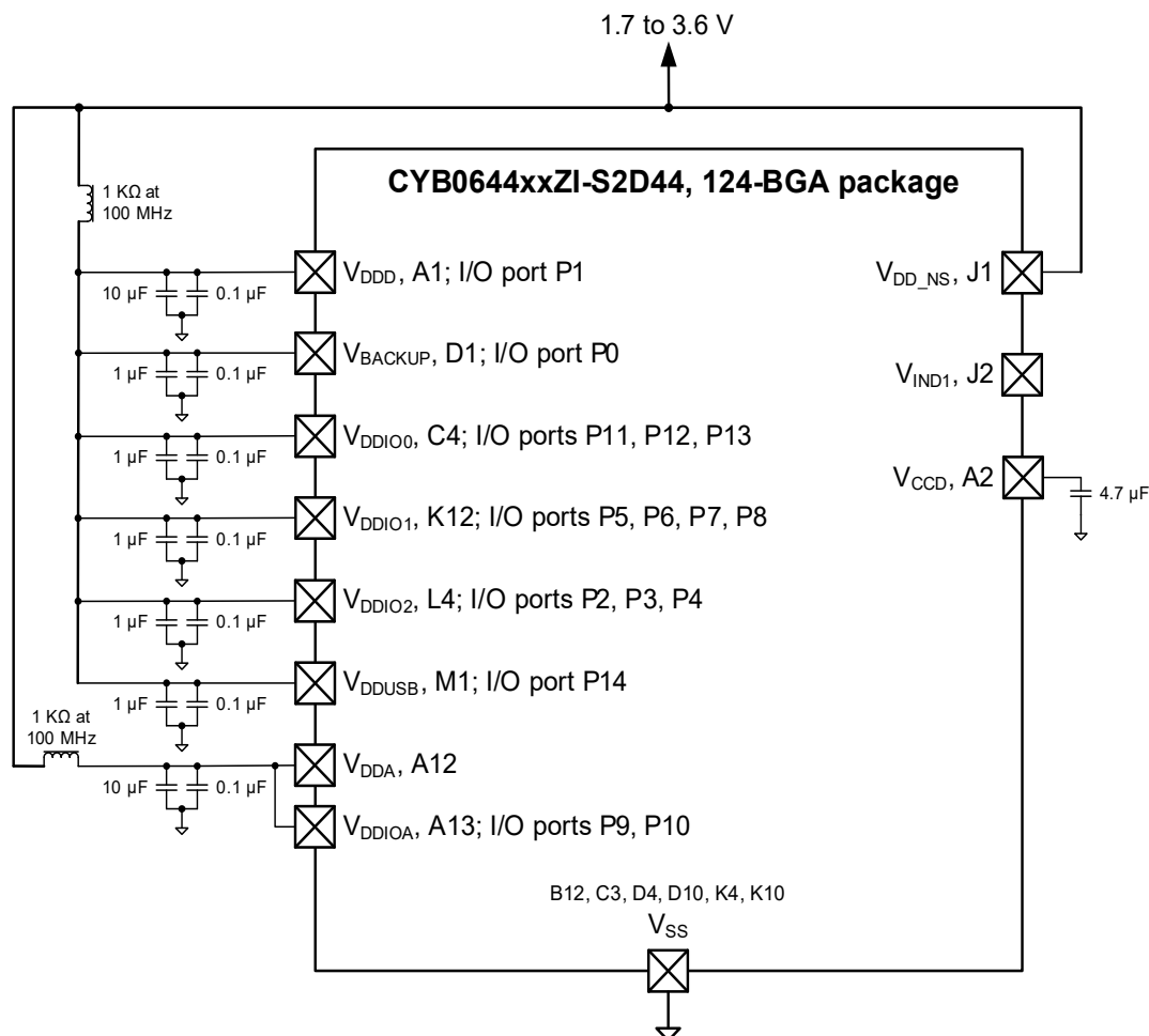
Figure 9. 124-BGA (No Buck) Power Connection Diagram
