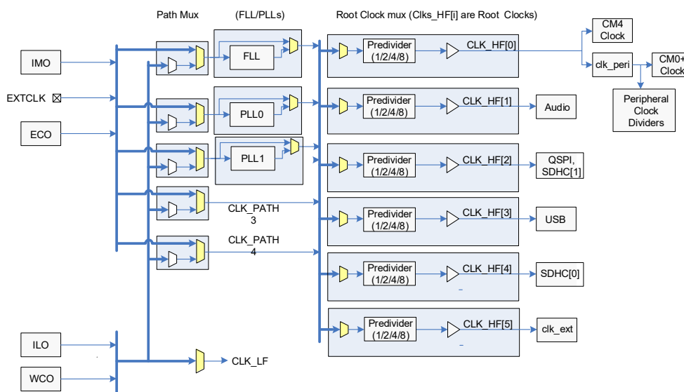
Figure 3. Clocking Diagram
