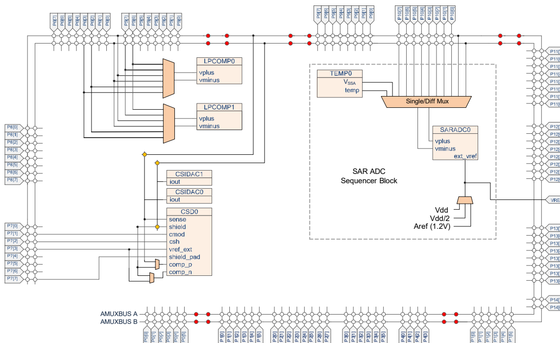
Figure 4. CYS0644xxZI-S2D44 Analog Subsystem
