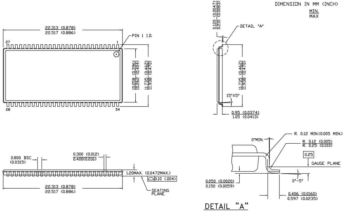
图 21. 54-pin TSOP II (22.4 x 11.84 x 1.0 mm) Z54-II 封装外形, 51-85160
