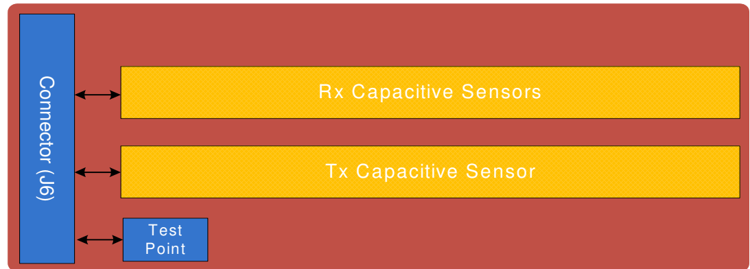
Liquid Level Sensor Flex
