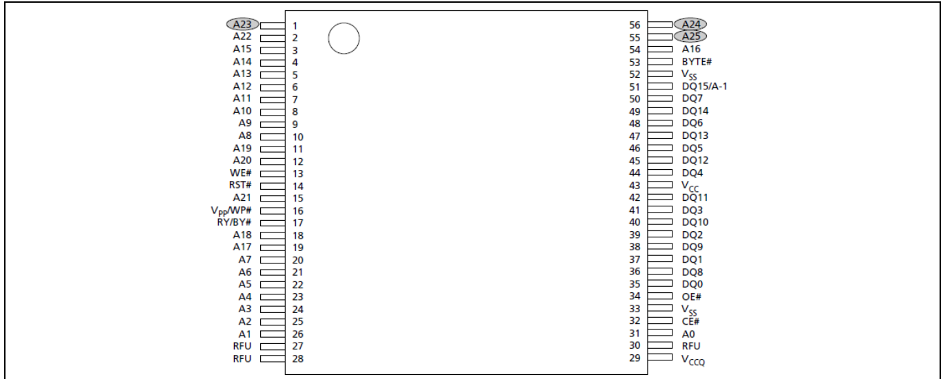
Figure 1 JS28FxxxM 56-Lead TSOP
