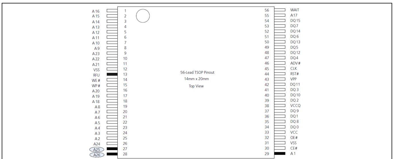
Figure 2 JS28FxxxM 56-Lead TSOP
