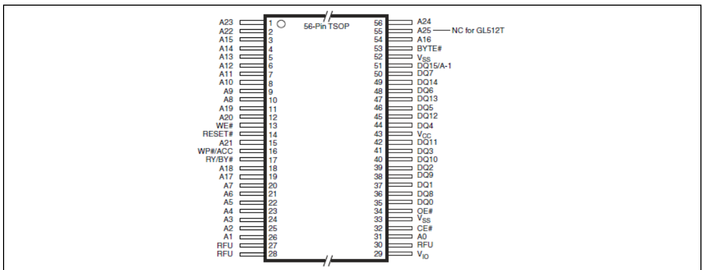
Figure 3 S29GL-S/S29GL-T 56-Lead TSOP
