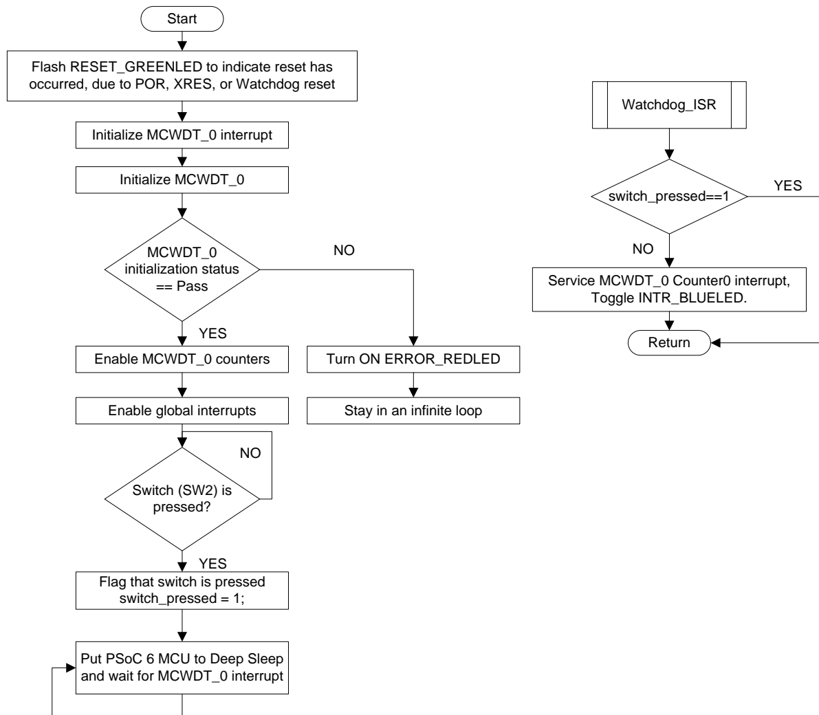
Figure 2. Firmware Flowchart
