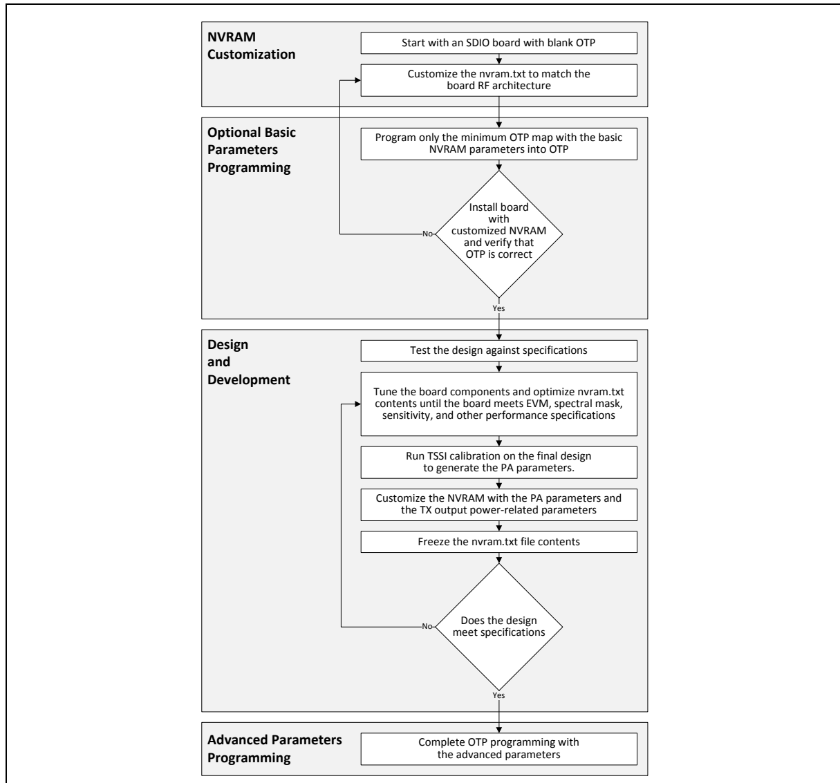
Figure 1. NVRAM Development and OTP Programming Flow
