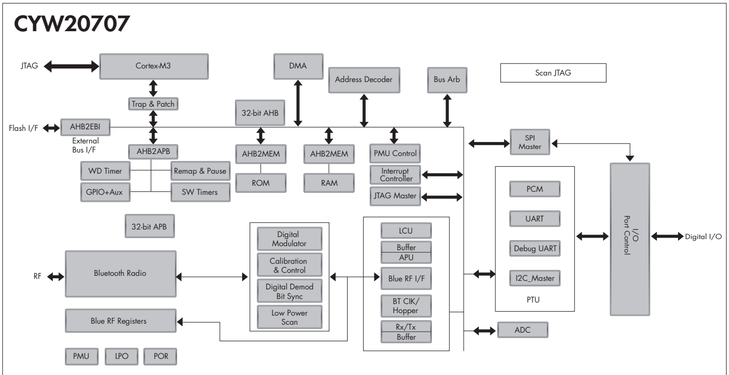
CYW20707 Functional Block Diagram
