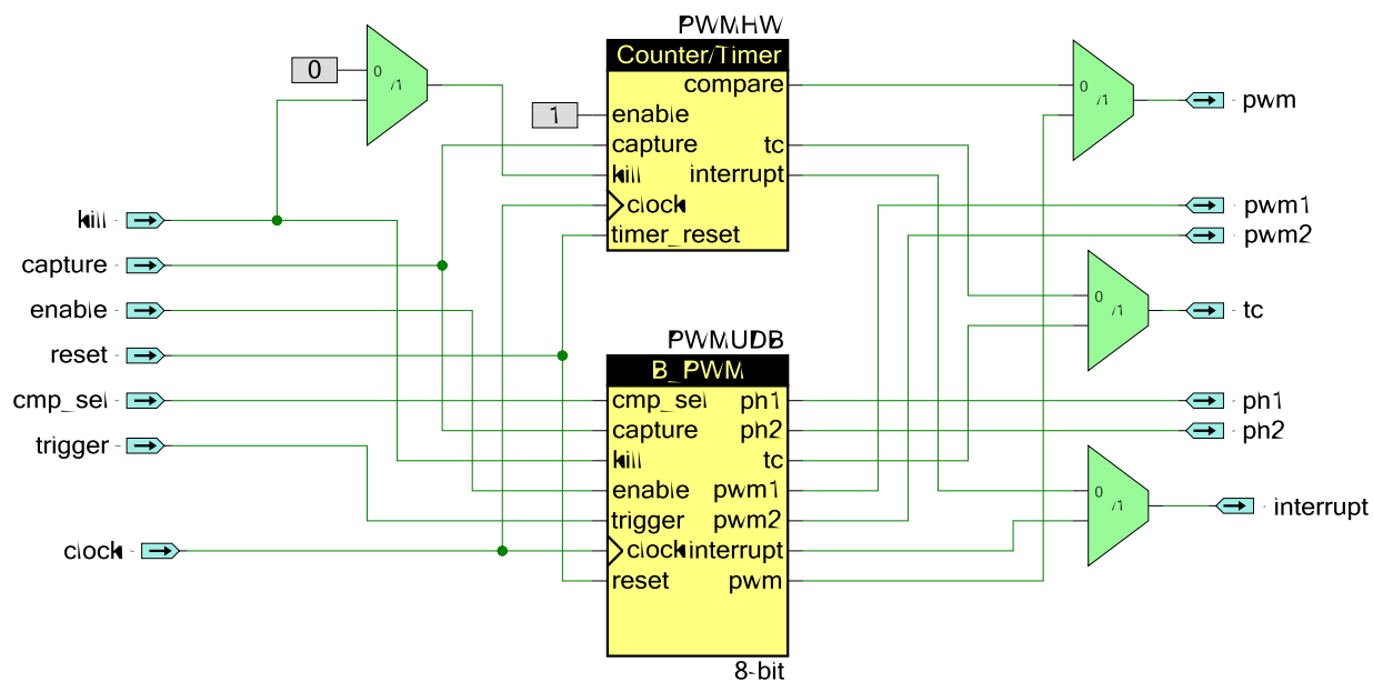
Figure 1. Top-Level Schematic
