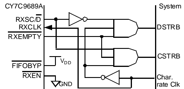
Figure 9. RXSC/D to DSTRB and CSTRB Translation
