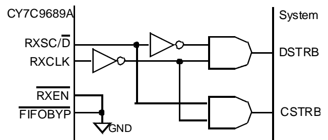
Figure 8. RXSC/D to DSTRB and CSTRB Translation
