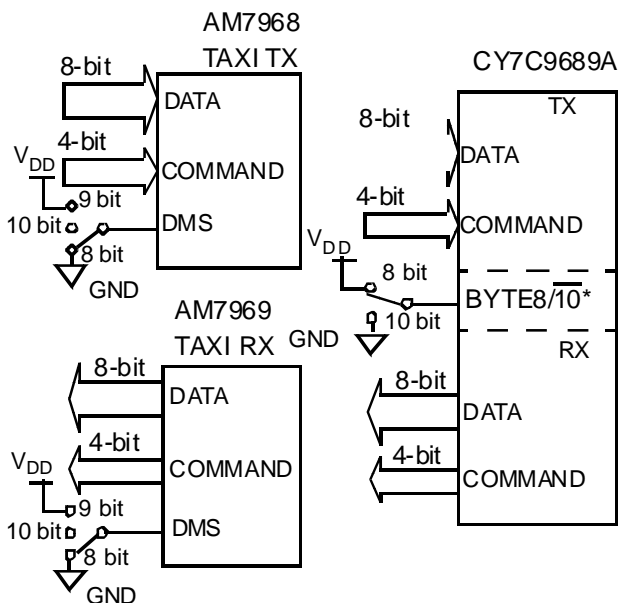
Figure 2. 8-bit Data Bus Configuration
