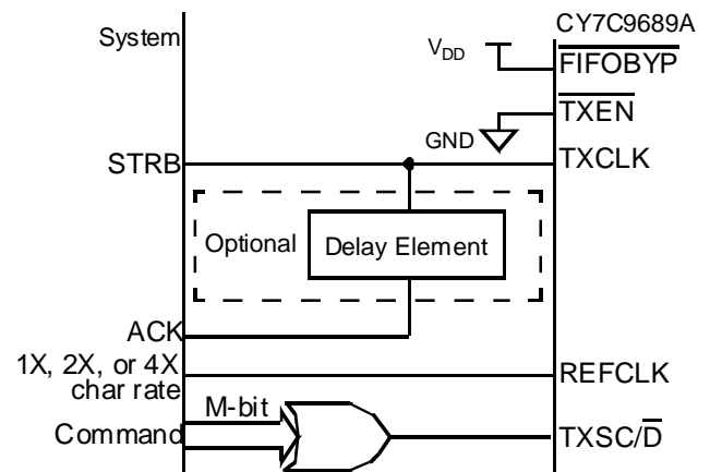
Figure 6. Asynchronous TX External Logic
