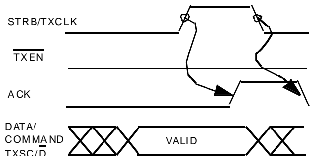
Figure 7. Asynchronous TX External Logic Timing
