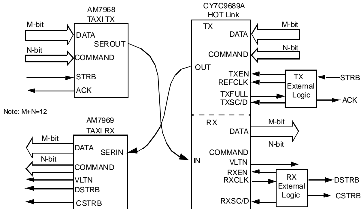
Figure 1. TAXI vs. CY7C9689A System Parallel Interface
