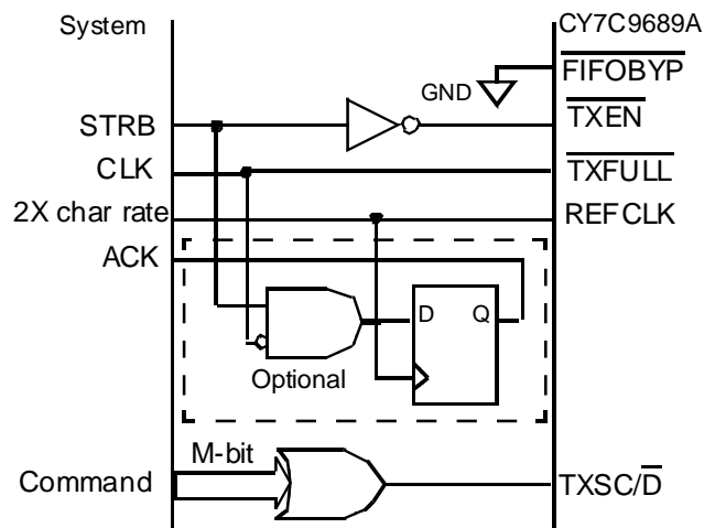
Figure 3. TX External Logic
