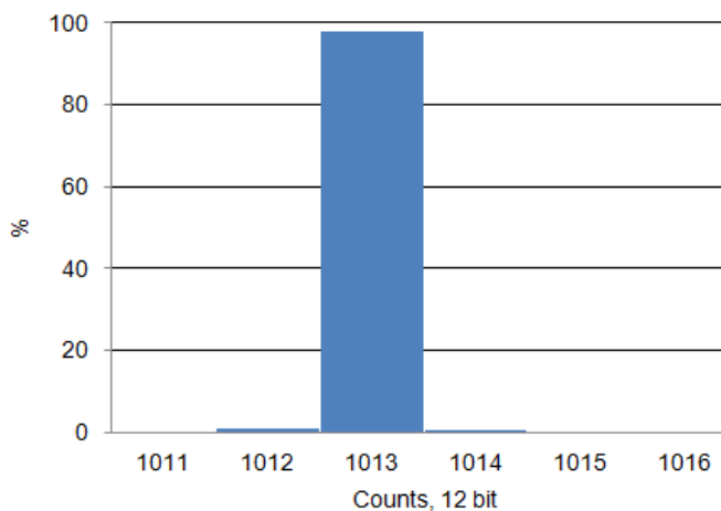
Noise Histogram, 1000 samples, 700 kbps, Internal Reference Bypassed, VIN = VREF/2
