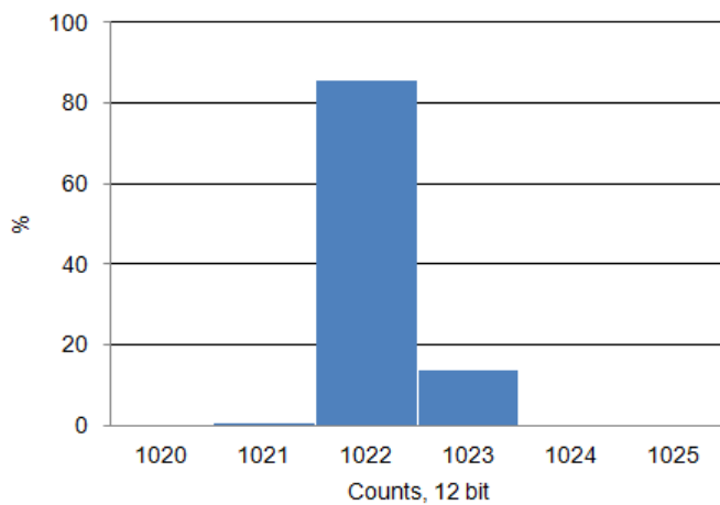
Noise Histogram, 1000 samples, 700 kbps, Internal Reference No Bypass, VIN = VREF/2
