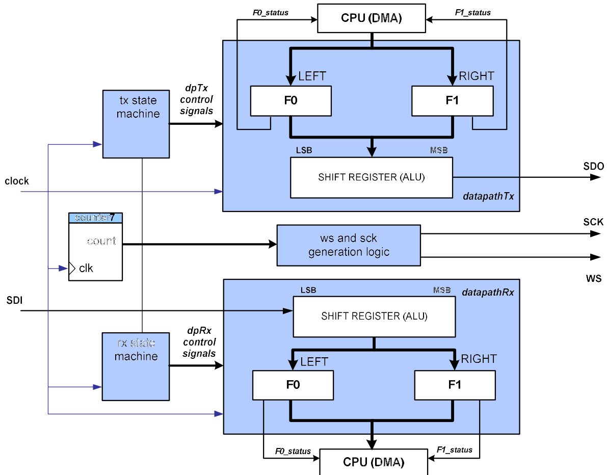
Figure 3. I2S Implementation
