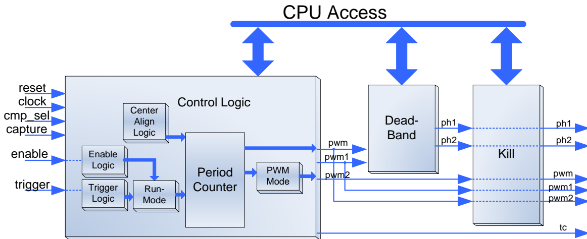
Figure 5. UDB Implementation
