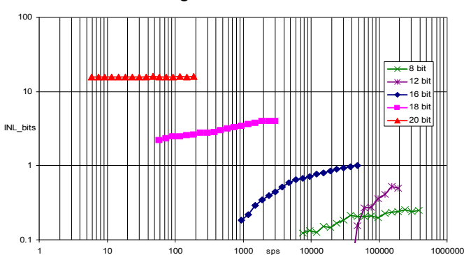
Integral Non Linearity, Range= \pm 1.024V
