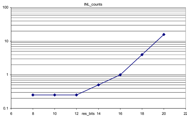
Integral Non Linearity, Range= \pm 1.024V
