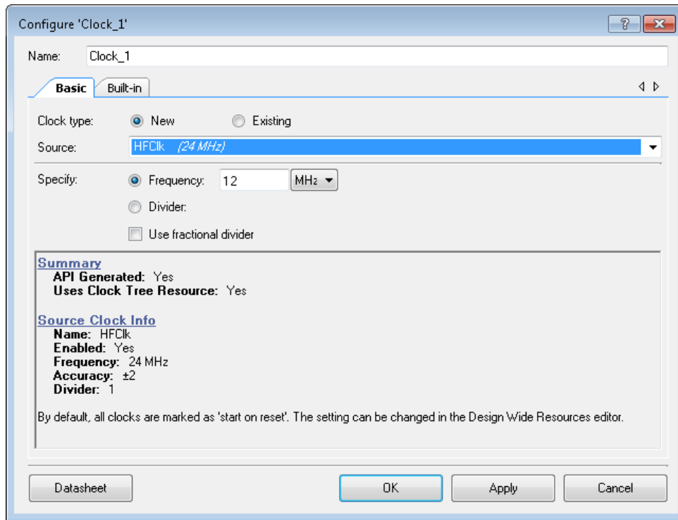
Figure 2. Clock Type: New / Source: Specific Clock
