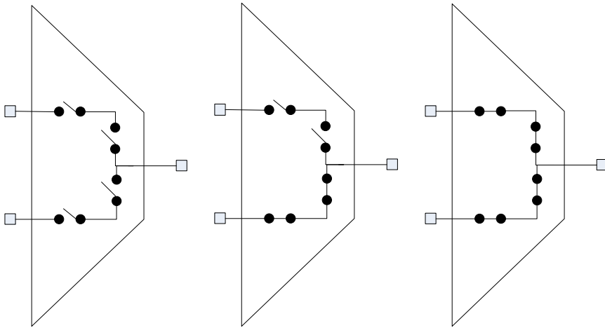
Figure 2. Double Switching, unique inner switches
