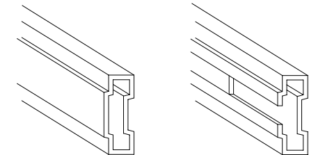
RED/BLACK SLOTTED TUBE PERSPECTIVE
