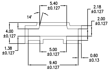
RIGHT SIDE VIEW (WITHOUT SLOT)
