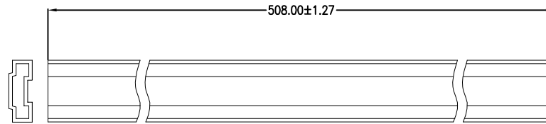
TOP VIEW (WITHOUT SLOT)
