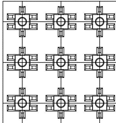
BOTTOM VIEW (SCALE:5/1)
