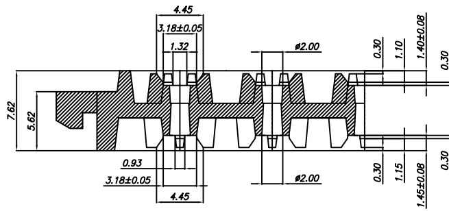
SECTION "A-A" (SCALE:5/1)
