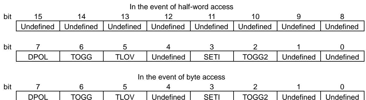
Figure 1-4. Bit structure of the hardware sequence flags
