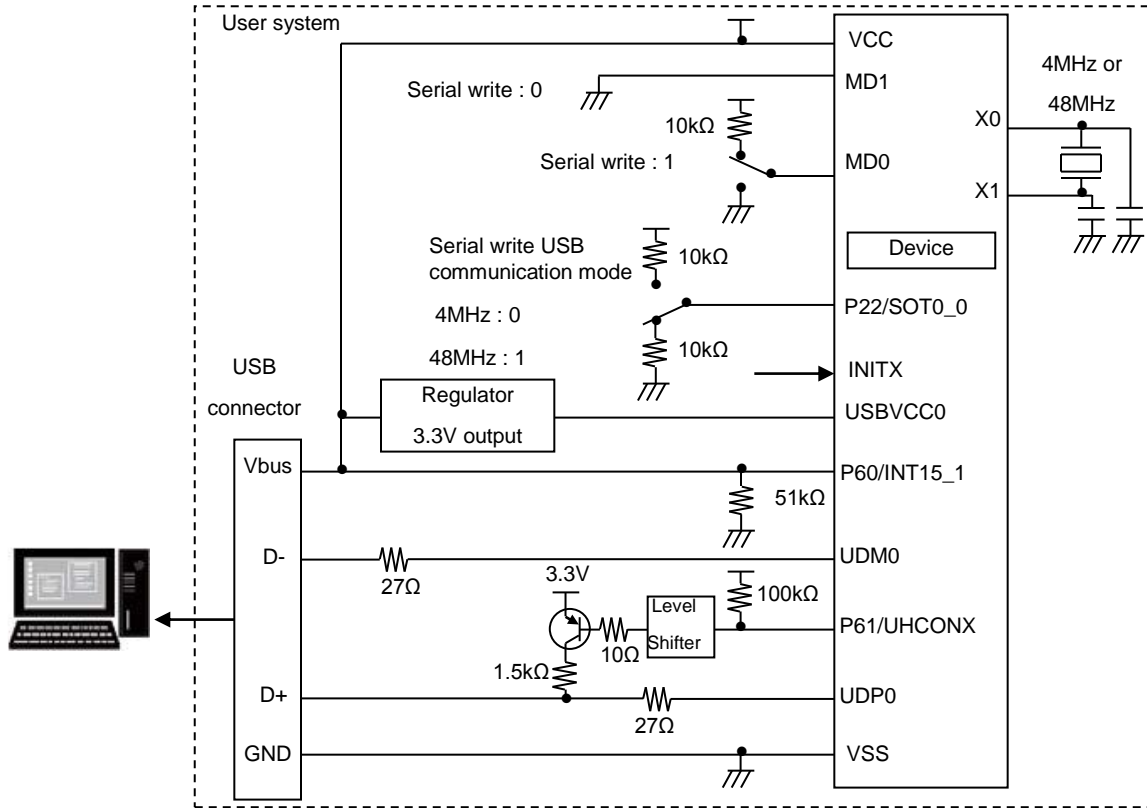
Figure 4-5. Connection example using CYPRESS USB DIRECT Programmer (bus power supply is used)
