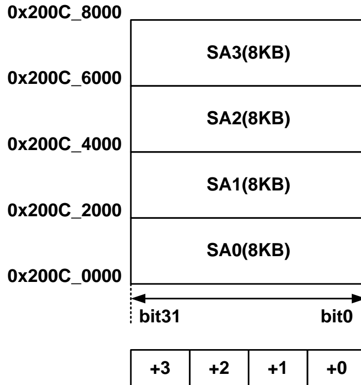
Figure 2-1. Memory map of WorkFlash memory
