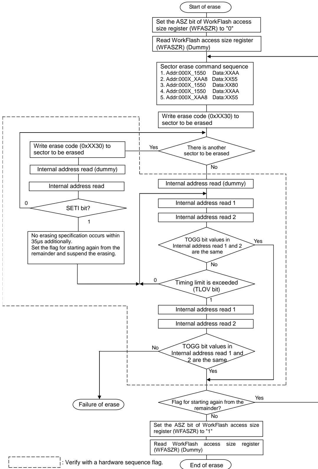
Figure 2-4. Example Sector Erase Procedure
