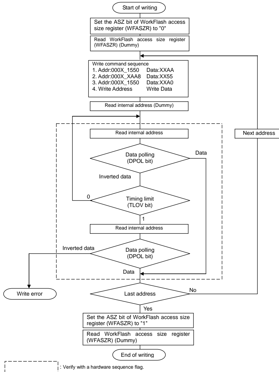
Figure 2-3. Example Write Operation
