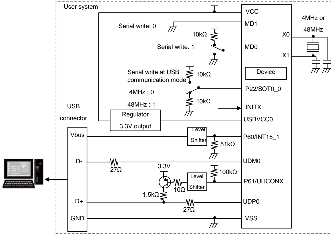
Figure 4-4. Connection example using CYPRESS USB DIRECT Programmer (own power supply is used)
