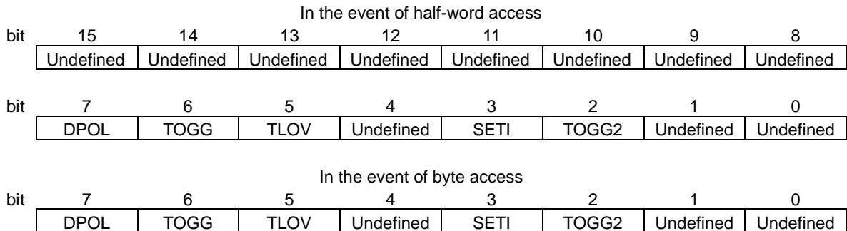
Figure 2-2. Bit structure of the hardware sequence flags
