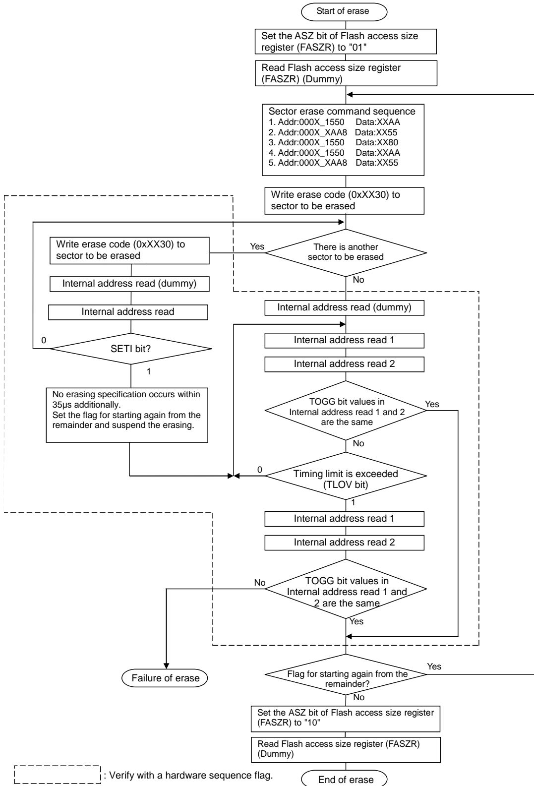
Figure 1-6. Example Sector Erase Procedure
