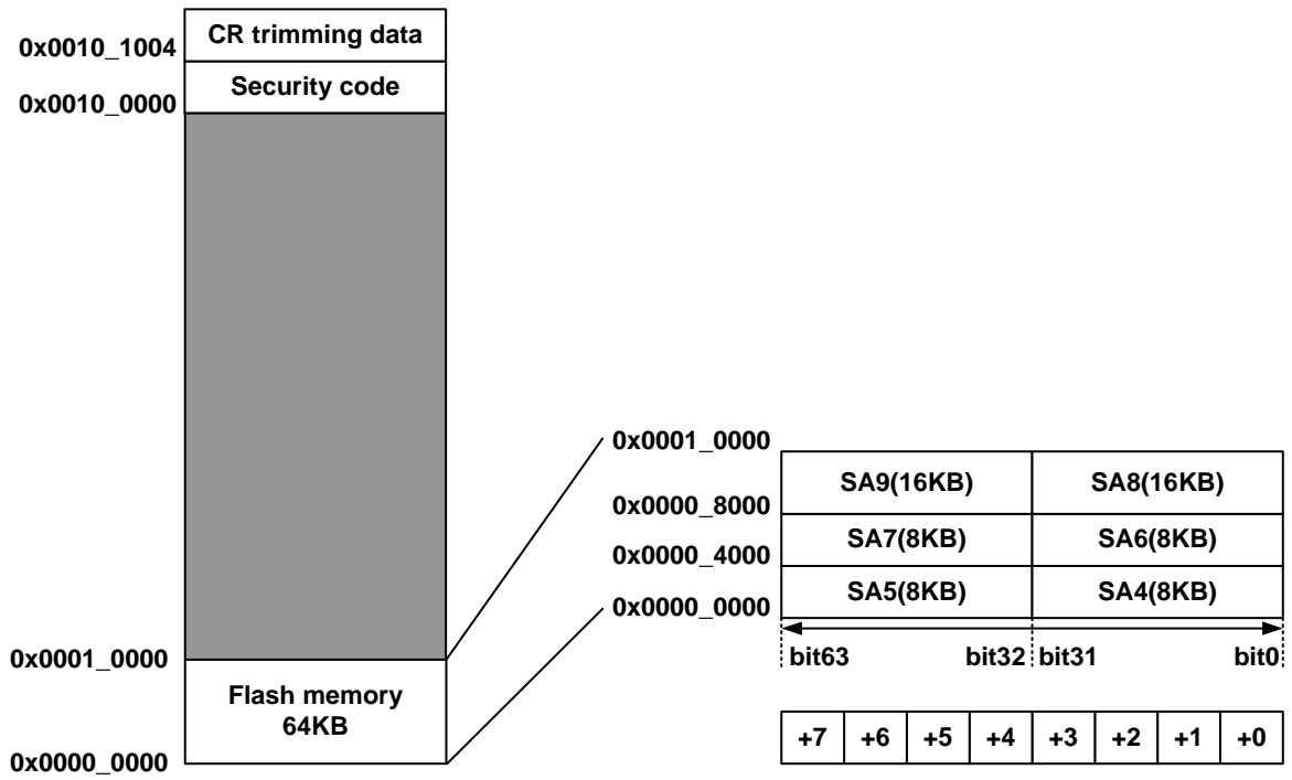
Figure 1-2. Memory map of M9AF112K/312K MainFlash memory
