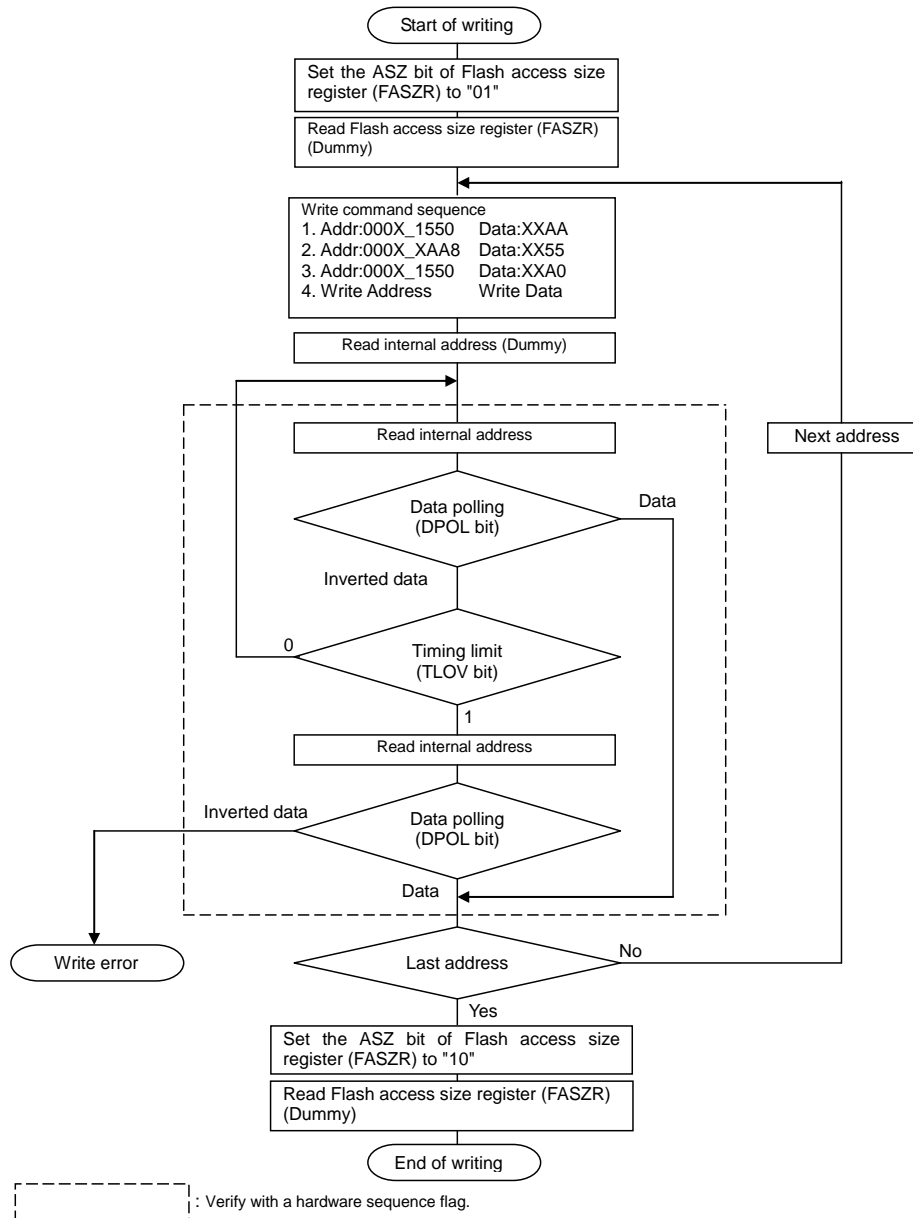
Figure 1-5. Example write operation
