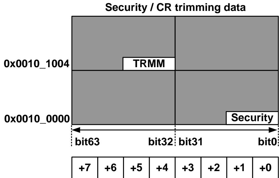
Figure 1-3. Address of Security/CR trimming data
