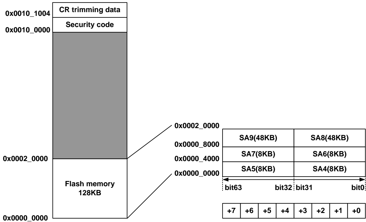
Figure 1-1. Memory map of M9AF111K/311K MainFlash memory
