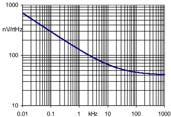
Input Voltage Noise Density T = 25 °C, V DDA = 5.0 V, Power = high
