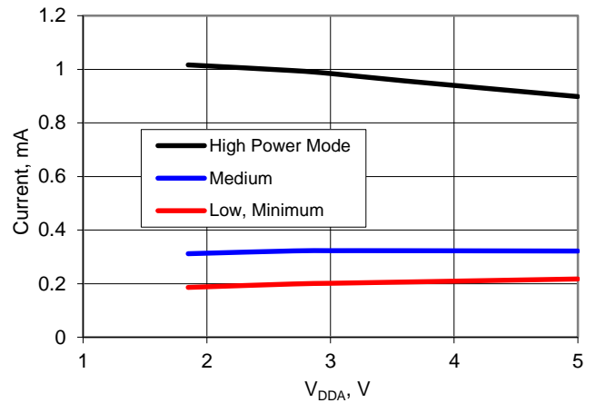
Operating Current versus Voltage T = 25 °C
