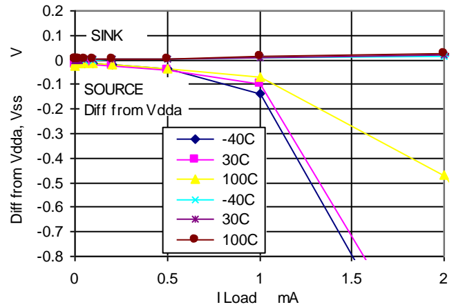
Output Voltage versus Load Current, V_{DDA} = 5.0 \text{ V} , Power = Low
