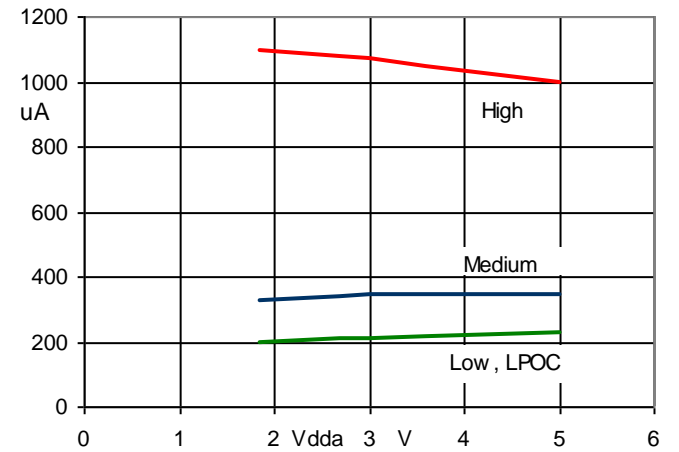
Operating Current versus Voltage T = 25 °C
